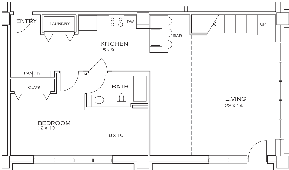
MAIN LEVEL
